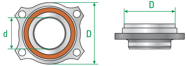
Radlager Generation 2D
