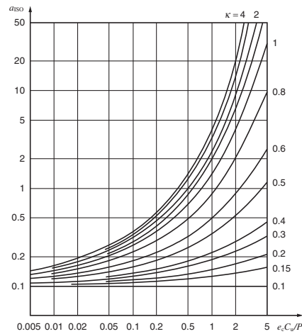
Fig. 1-5 Life modification factor a_{ISO} (Thrust roller bearings)
