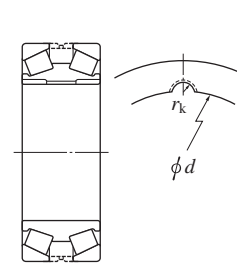
Bore key way
