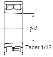
Tapered bore
